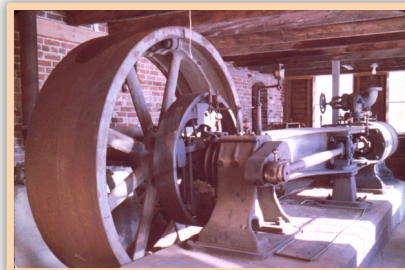
1890's Fitchburg Steam Engine
